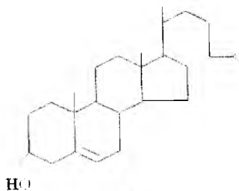
Xolesterin (C 27 )
