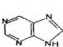
Purin
