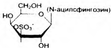
Sulfolipid
