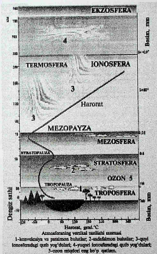
8.1-rasm. Atmosferaning vertikal tuzilishi (R.Ramade, 1998 y).
