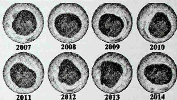
8.4-rasm. Ozon qatlamining hozirgi holati (Levashov, 2015)
