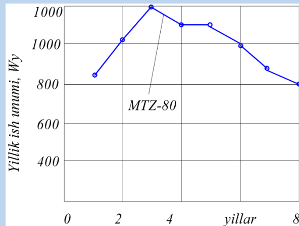
77-rasm. MTZ-80 transport traktori yillik ish unumining foydalanish jarayonida o'zgarish grafigi
